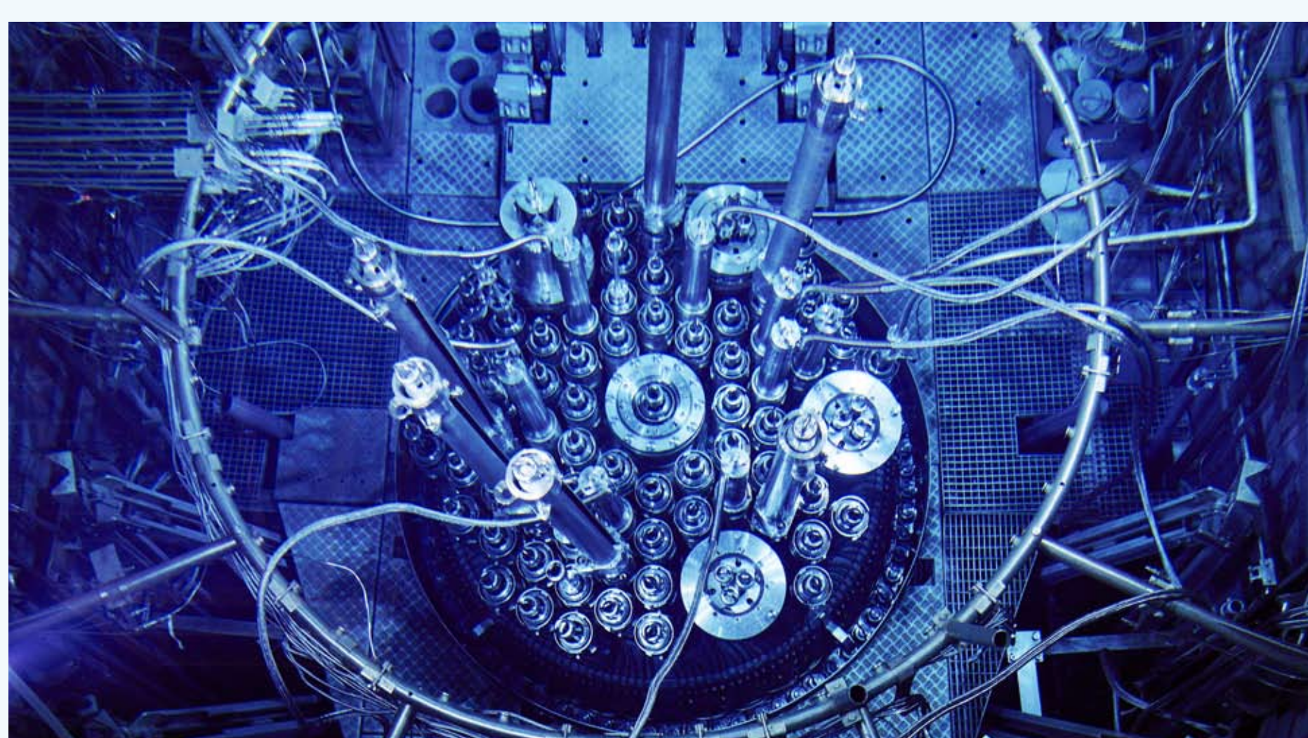
BR2 research reactor at SCK CEN, Mol, Belgium Source: SCK CEN. Used by permission
